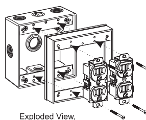
Exploded View, EXR-2 Shown Installed
