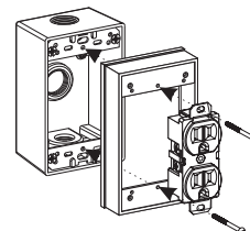
Exploded View, EXR-1 Shown Installed
