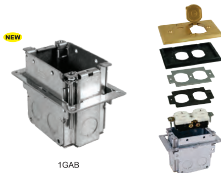
EXPLODED DRAWING FLB Series
