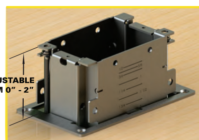
SUB-FLOOR INSTALLATION
