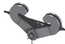
FIG. 450 HEAVY BEAM CLAMP ASSEMBLY
