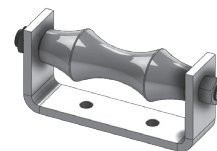
FIG. 275 ROLLER CHAIR
