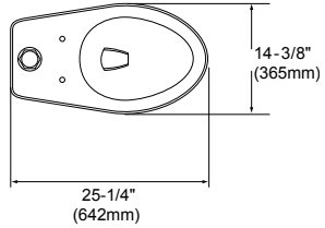
12" rough-in dimensions
