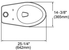
12" rough-in dimensions
