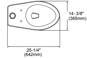
12" rough-in dimensions
